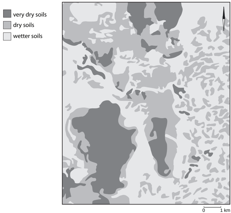
Figure 9.16 Groundwater classes in the Borkeld study area.
